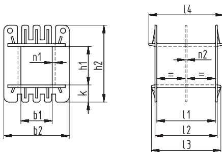
Sketch with main dimensions
