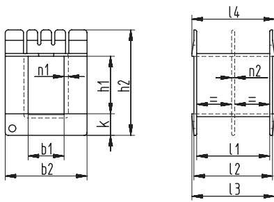
Sketch with main dimensions
