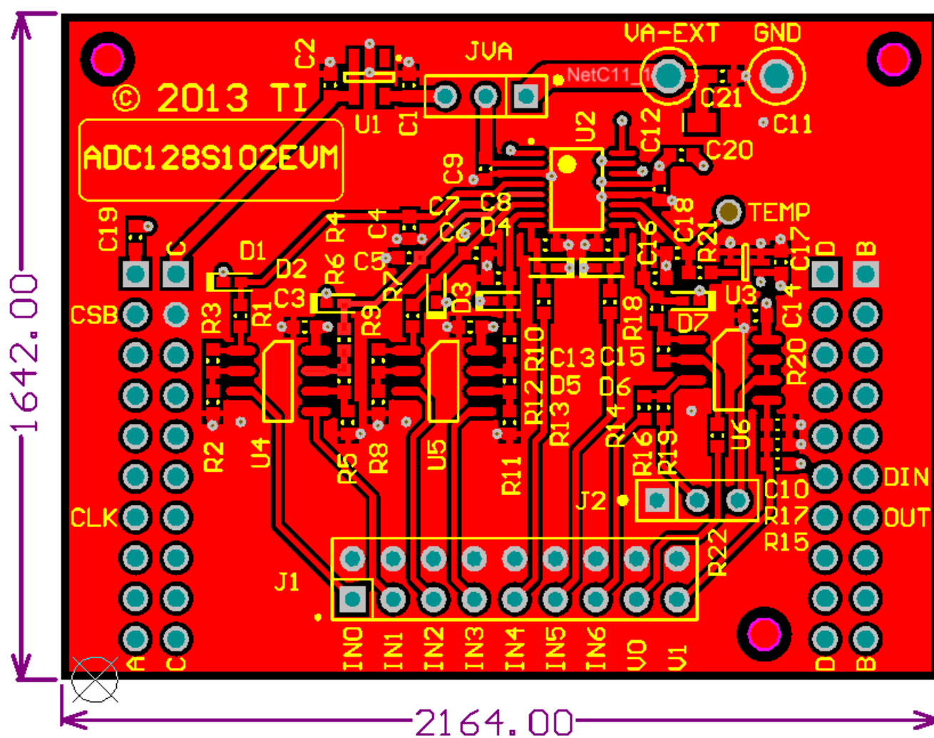
Figure 4-1. Top Assembly Layer
