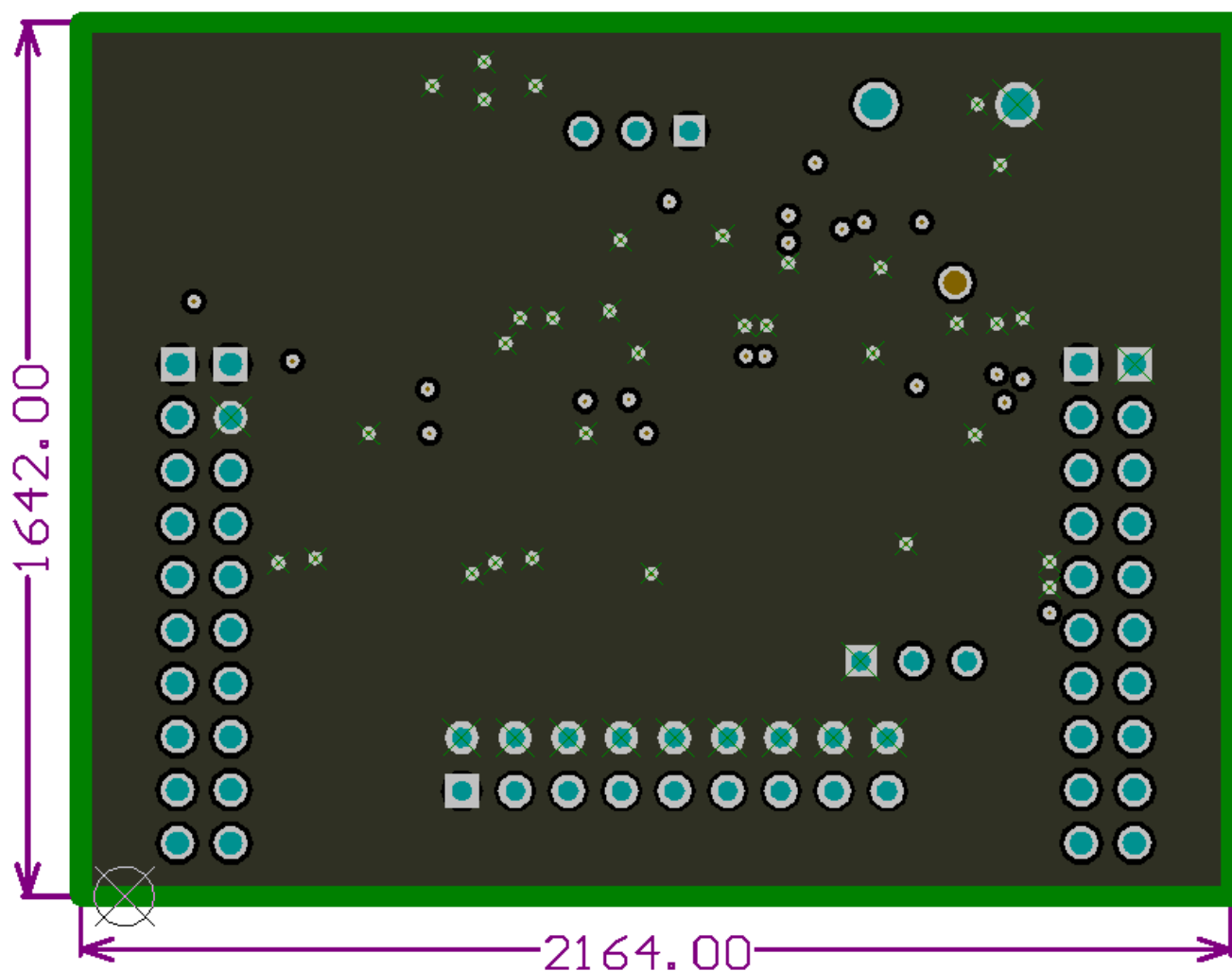
Figure 4-4. Ground Layer Routing
