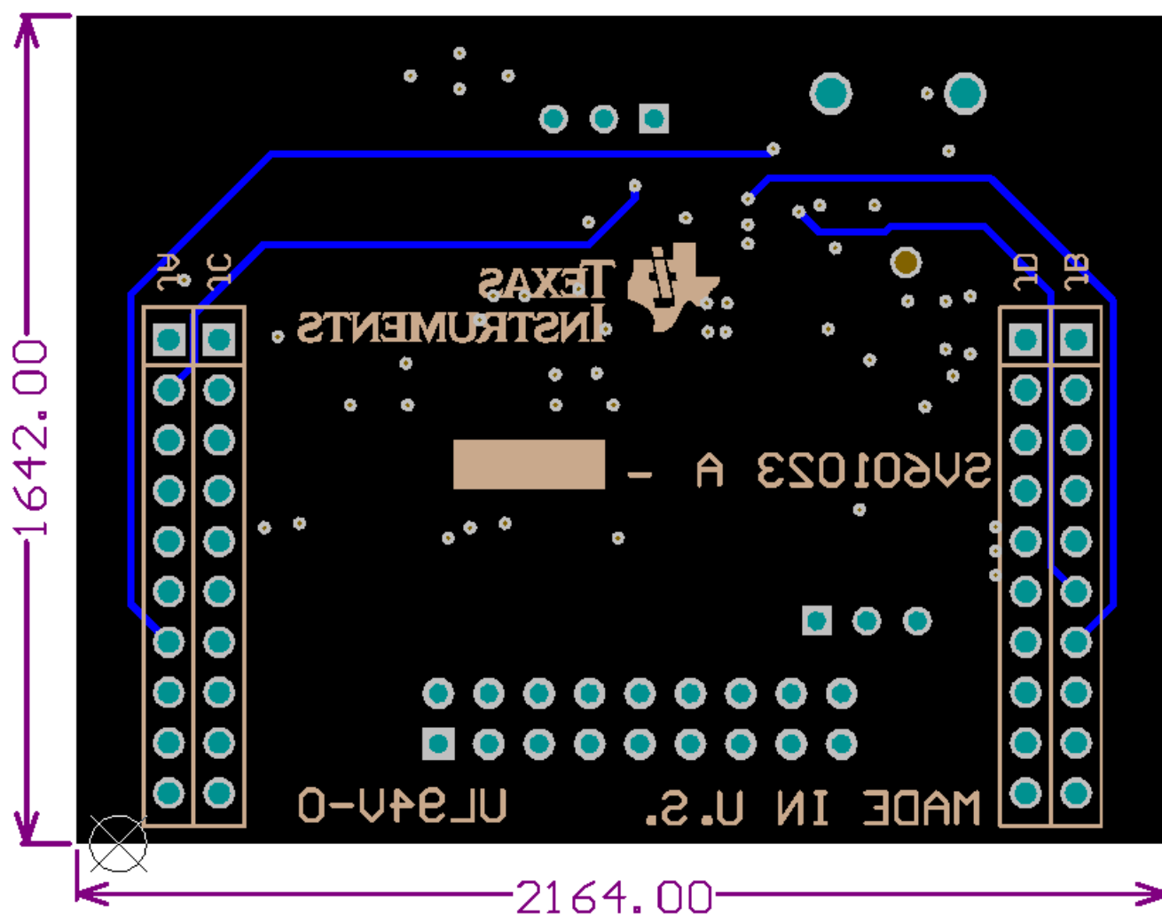
Figure 4-5. Bottom Layer Routing
