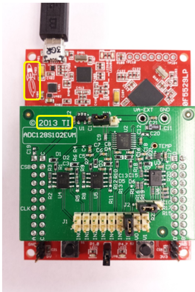
Figure 3-1. ADC128S102EVM Attached to MSP430
