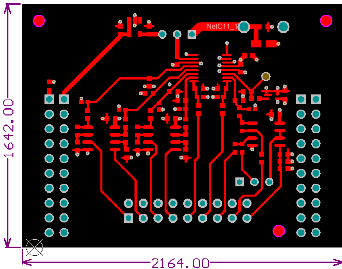
Figure 4-2. Top Layer Routing
