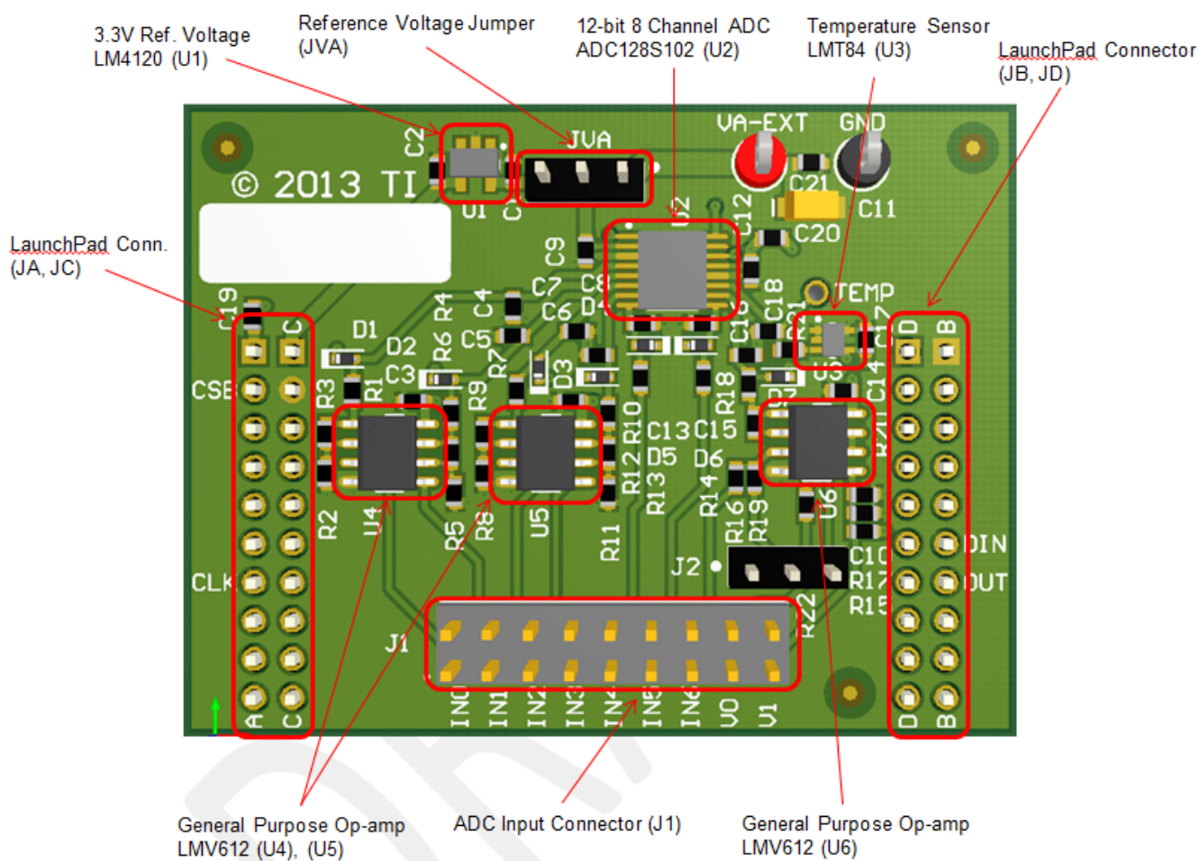
Figure 1-1. ADC128S102EVM Evaluation Board
