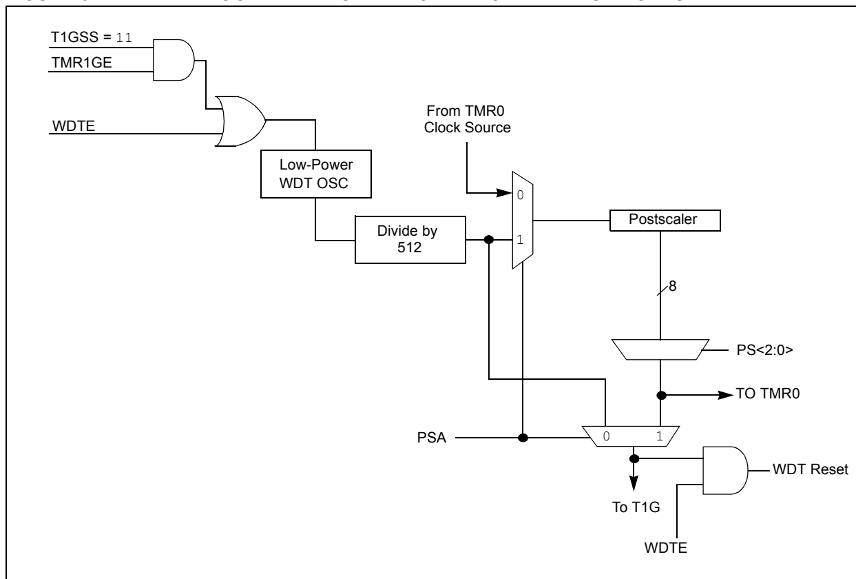
FIGURE 3-1: WATCHDOG TIMER BLOCK DIAGRAM FOR WDT TEST MODES
