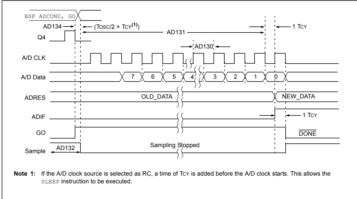
FIGURE 23-13: PIC16F72X A/D CONVERSION TIMING (SLEEP MODE)
