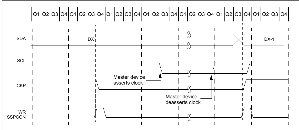
FIGURE 17-13: CLOCK SYNCHRONIZATION TIMING
