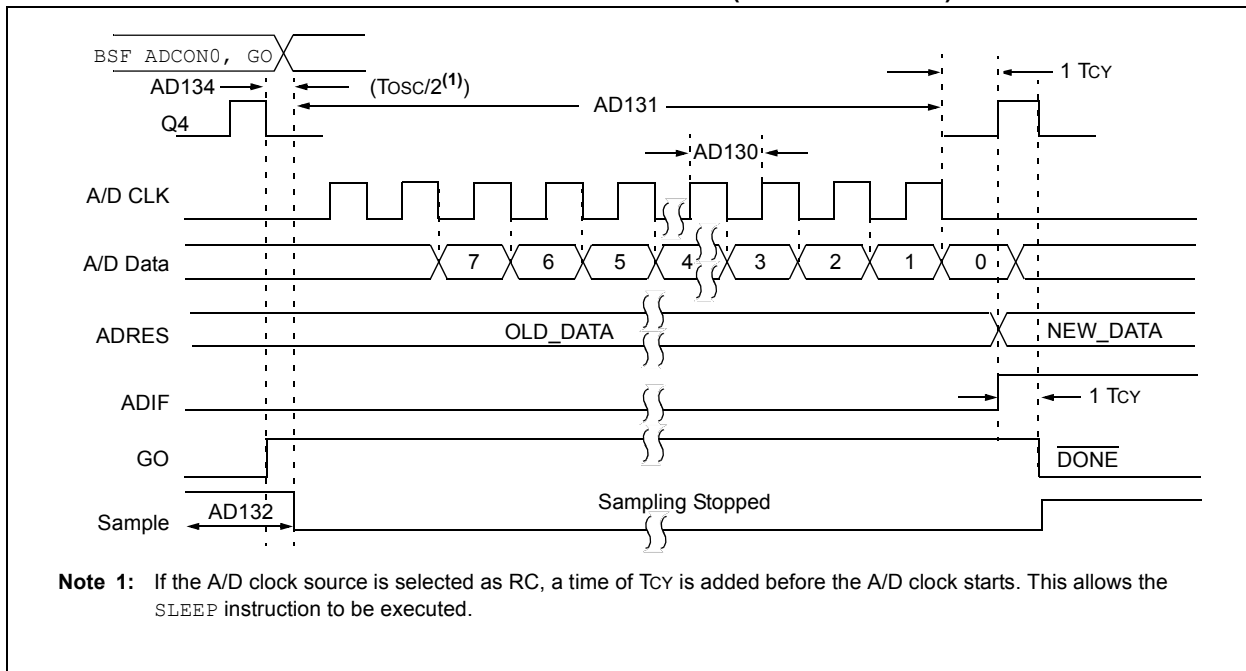
FIGURE 23-12: PIC16F72X A/D CONVERSION TIMING (NORMAL MODE)
