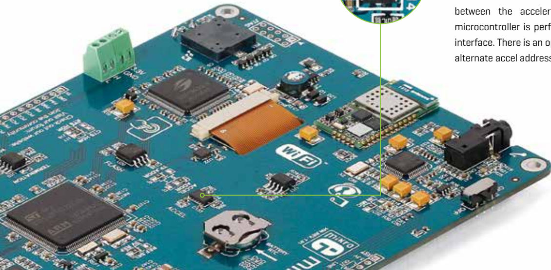
Figure 11-1: Accelerometer module
