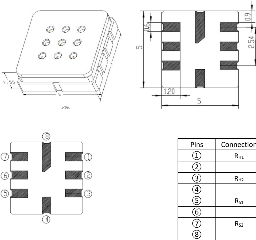
Fig1.Sensor structure
