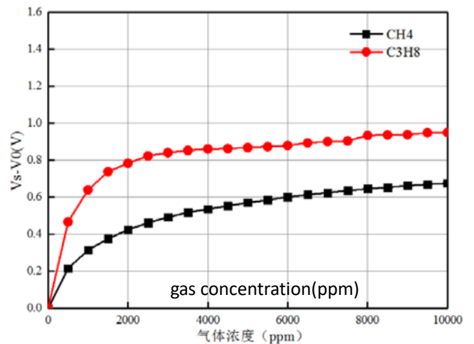
Fig6. Linearity character
