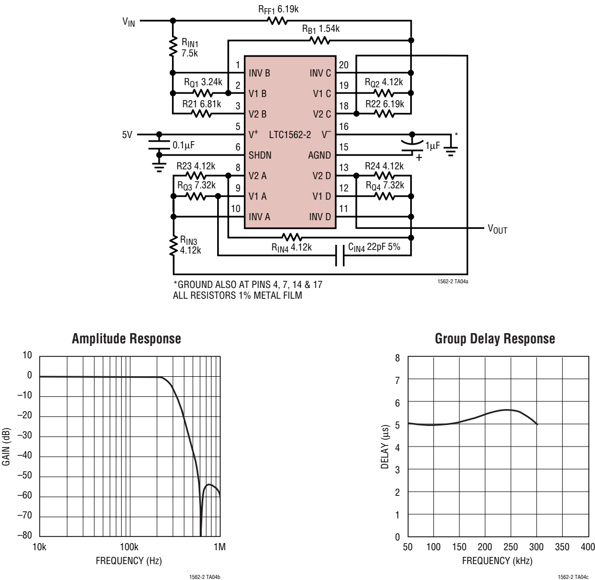
256kHz Linear Phase 6th Order Lowpass Filter with a 2nd Order Allpass Phase Equalizer, Single Supply
