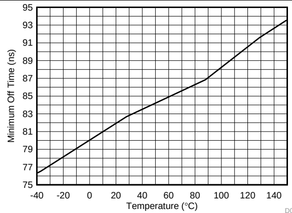
Figure 2. Minimum Off-Time vs Temperature
