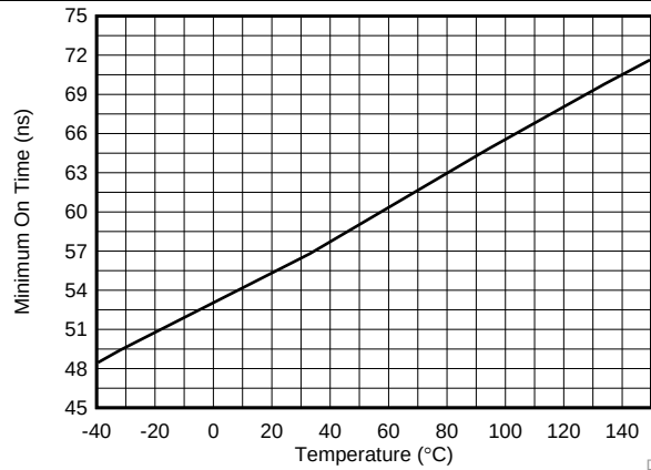
Figure 1. Minimum On-Time vs Temperature
