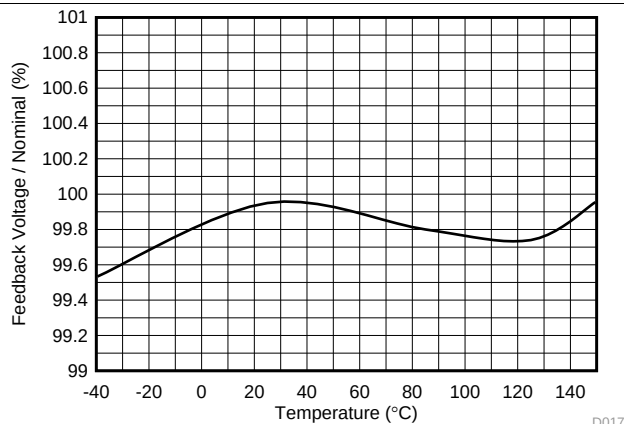
Figure 5. Normalized V_{FB} vs Temperature
