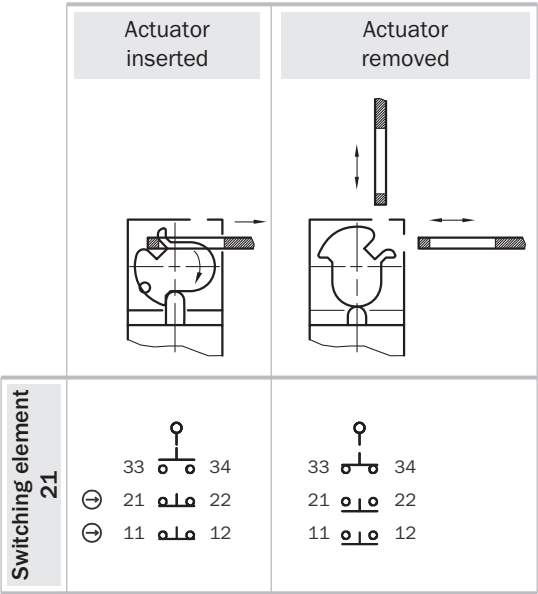
Switching element 21: 2 positive action N/C contacts + 1 N/O contact
