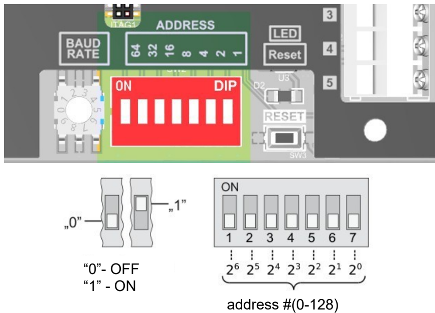
Figure 3. Transmitter addressing.
