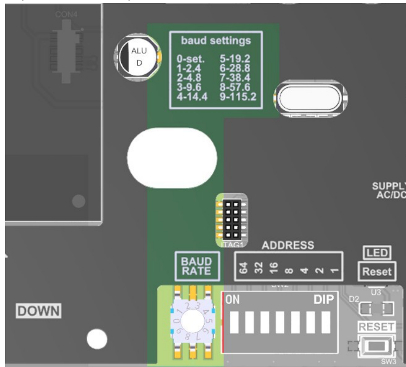
Figure 4. RS-485 interface speed setup.
