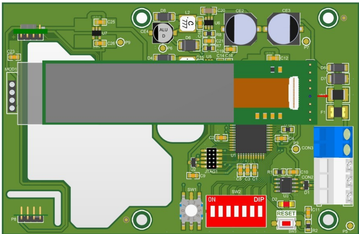
Figure 1. View of the transmitter PCB.
