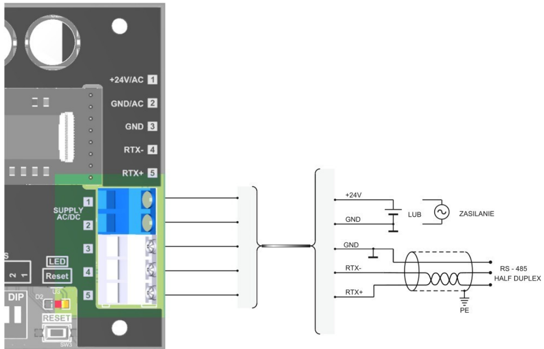
Figure 2. Transmitter connection diagram
