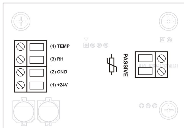
Figure 1. Outs Description of the HCRH2xKb Series Sensor
