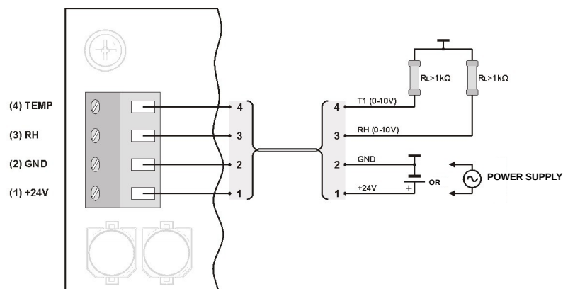
Figure 1. Outs Description of the HCRH2xKb Series Sensor
