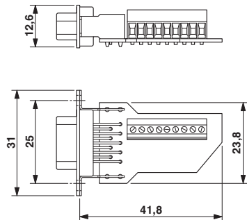
Dimensional drawing
