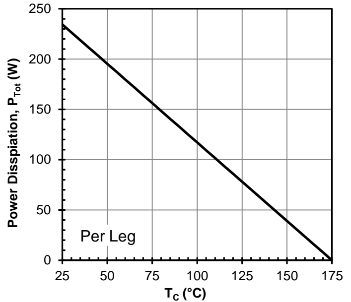
Figure 4 Power dissipation
