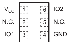
DRY Package 6-Pin USON Top View
