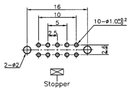
P.C.B. MOUNTING DETAIL
