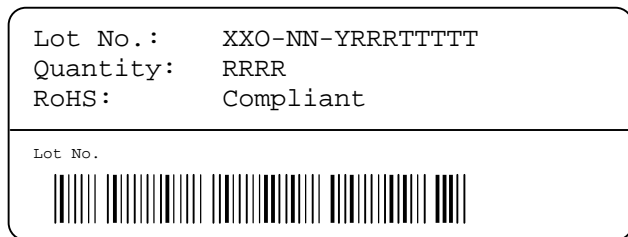
Figure 13: First label on reel: XX = Sensor Type (21 for SHT21), O = Output mode (D = Digital, P = PWM, S = SDM), NN = Chip Version, Y = last digit of year, RRR = number of sensors on reel divided by 10 (200 for 2000 units), TTTTT = Traceability Code.
