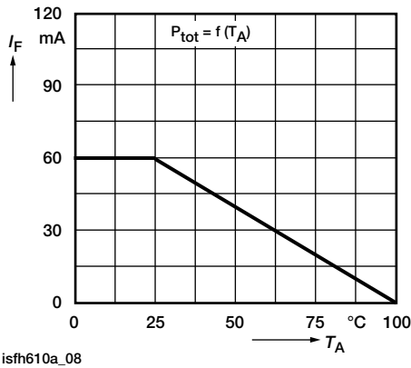
Fig. 8 - Permissible Power Dissipation vs. Temperature
