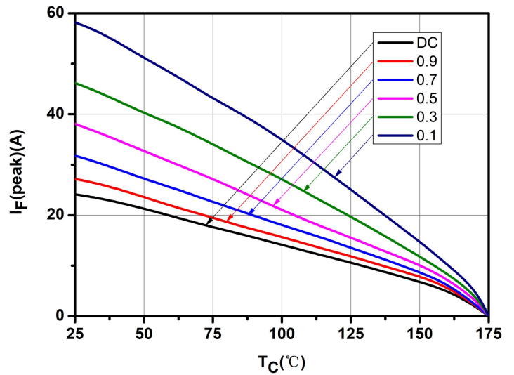
Fig.8-Current Derating
