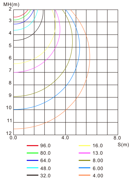
Spacing iso-illuminance curve
