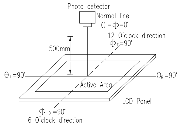
Fig.10.2. Optical measurement system setup
