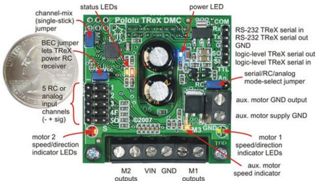
Pololu TReX Dual Motor Controller with labels
