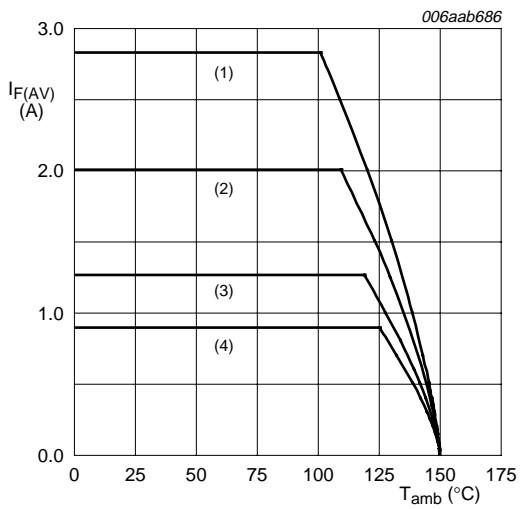
Ceramic PCB, Al_2O_3 , standard footprint T_j = 150\text{ }^\circ\text{C} (1) \delta = 1; DC (2) \delta = 0.5; f = 20\text{ kHz} (3) \delta = 0.2; f = 20\text{ kHz} (4) \delta = 0.1; f = 20\text{ kHz}
