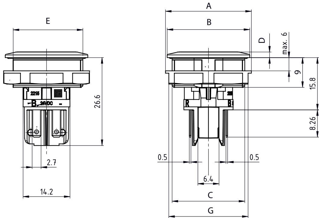
MSM II Indicator with Quick Solder Terminal
