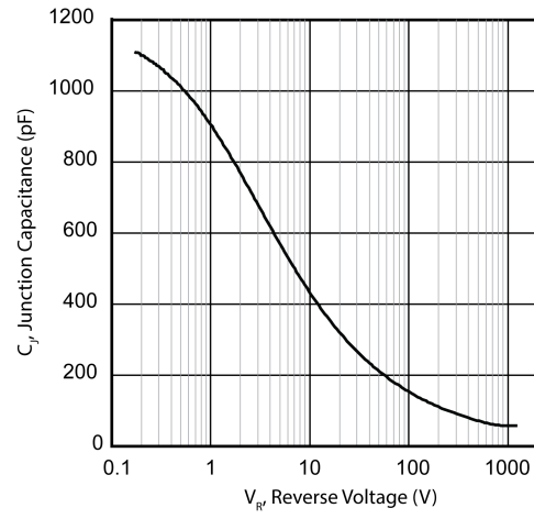
Figure 7 • Capacitance vs. Reverse Voltage
