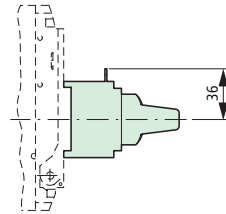
NZM1-XDTV
