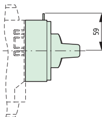
NZM2-XDTV NZM2-XDTV2
