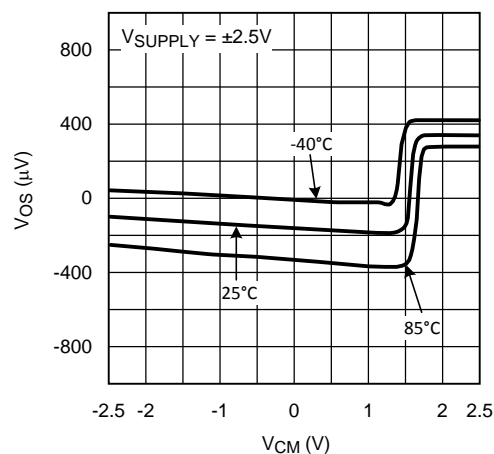
Figure 3. V_{OS} vs. V_{CM}
