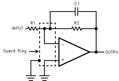
Figure 25. Inverting Amplifier
