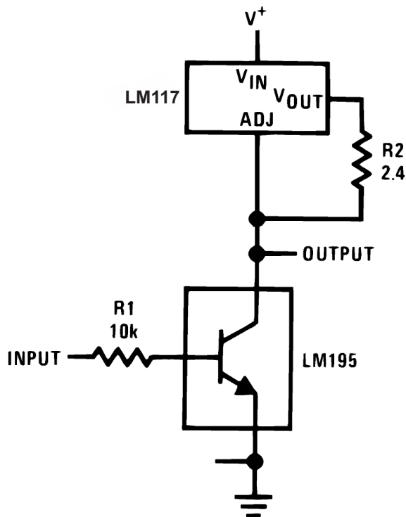
Figure 27. Common-Emitter Amplifier
