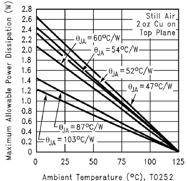
Figure 44. Maximum Allowable Power Dissipation vs Ambient Temperature for TO-252
