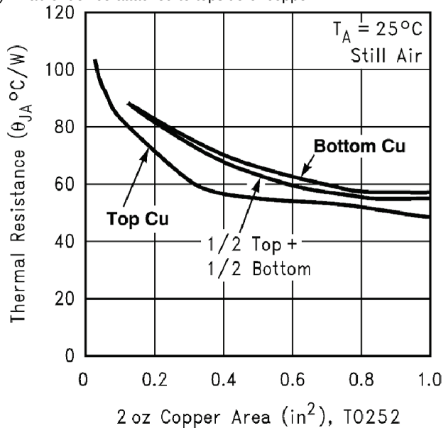
Figure 43. \theta_{JA} vs 2-oz. Copper Area for TO-252
