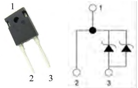
TO-247-2L
