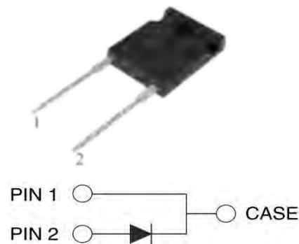
TO-247-2L
