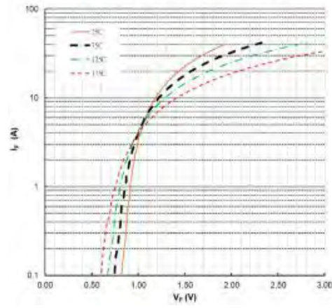
Figure 2. Forward Characteristics
