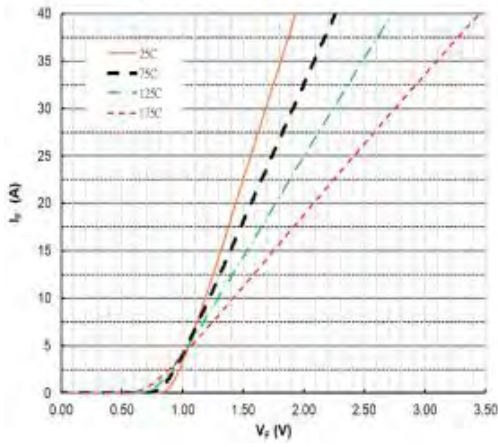
Figure 1. Forward Characteristics
