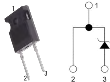
TO-247-2L
