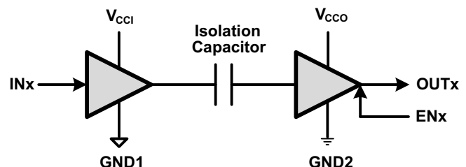
Simplified Schematic
