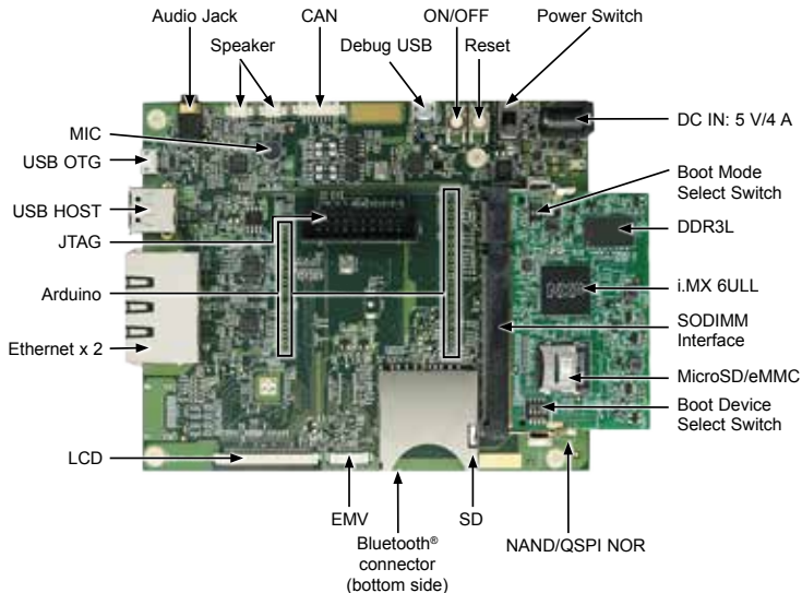
Figure 1: Main interfaces of i.MX 6ULL EVK
