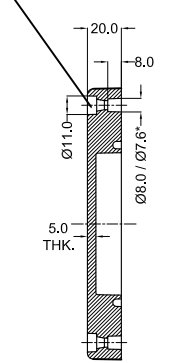
SECTION C-C
