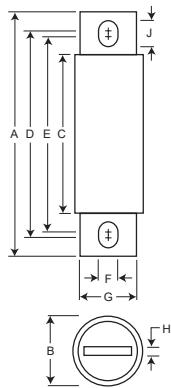
Fig. 1: 5-800 Amp Range
