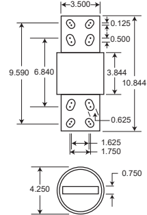
Fig. 3: 1200 Amp Range
