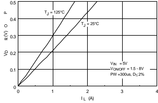
Figure 2. V_{DROP} Versus I_L at V_{IN}=5.0\text{V} .
