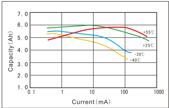
Capacity vs Current curve(cut off with 2.0V)
