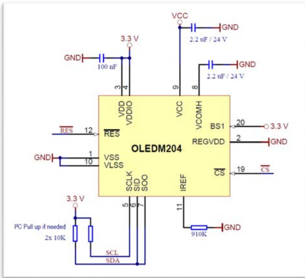
I2C - 3.3V - Address 0x78 (0x3C)
