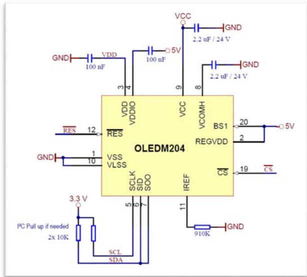
I2C - 5V - Address 0x78 (0x3C)
