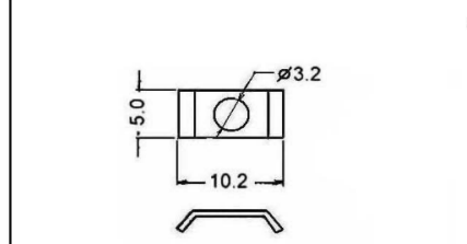
WASHER: STEEL IN NICKEL PLATED (2 pcs)
