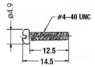
FIXED SCREW: STEEL IN NICKEL PLATED PHILLIPS HEAD (2 pcs)
