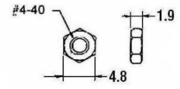
NUT: STEEL IN NICKEL PLATED (2 pcs)
