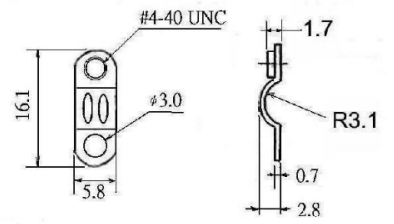
CABLE CLAMP: STEEL IN NICKEL PLATED (2 pcs)
