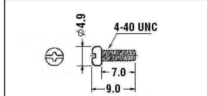
SCREW: STEEL IN NICKEL PLATED (2 pcs)
