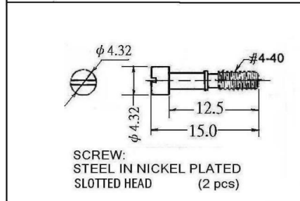
SCREW: STEEL IN NICKEL PLATED (2 pcs)
