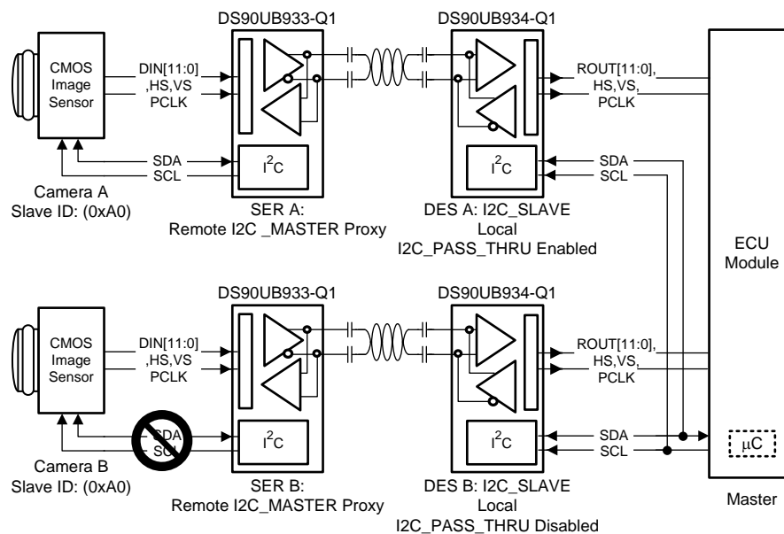
Figure 25. I2C Pass-Through
