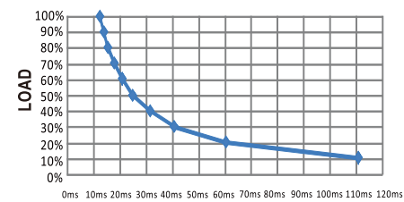
TIME (figure 6)
