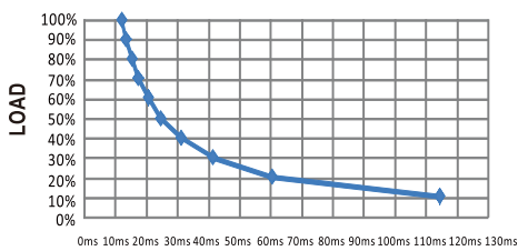
TIME (figure 5)
