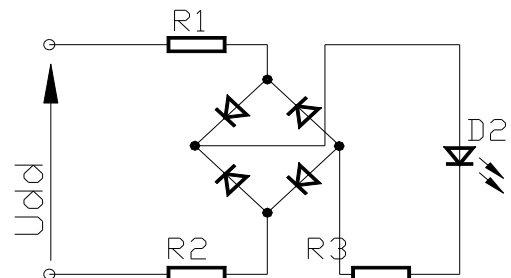
Full-wave rectifier
