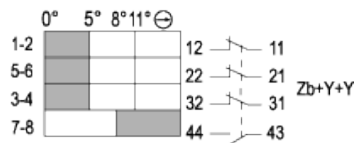
Travel diagram 1NO+3NC (Production setting)
