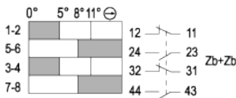
Travel diagram 2NO+2NC (Production setting)
