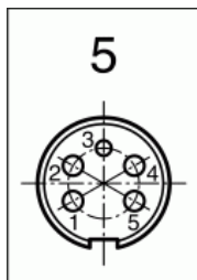
Contact arrangement
