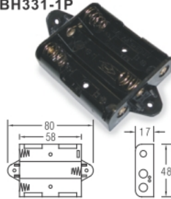
BH331-1A BH331-1B FOR THREE "AA" CELLS BH331-1D BH331-1P
