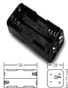
BH343-2A BH343-2B FOR FOUR "AA" CELLS BH343-2D
