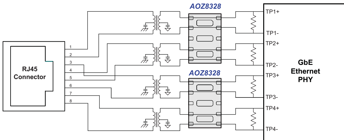
Figure 1. 10/100/1000 Ethernet Port Connection
