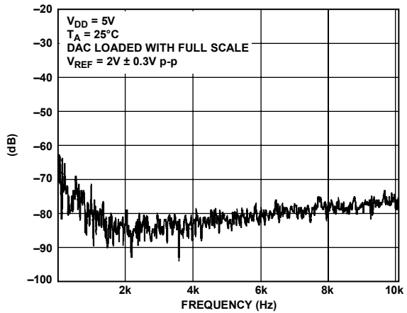
Figure 49. Total Harmonic Distortion
