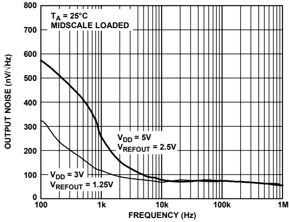
Figure 48. Noise Spectral Density, Internal Reference
