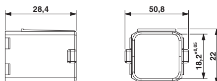
Dimensional drawing
